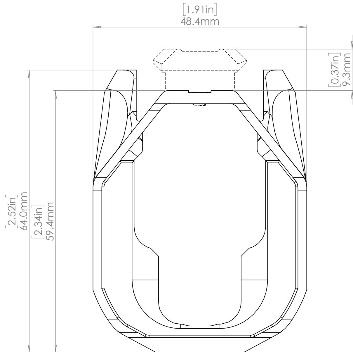
7-SLOT RAIL
