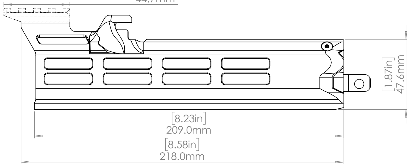
4-SLOT RAIL
