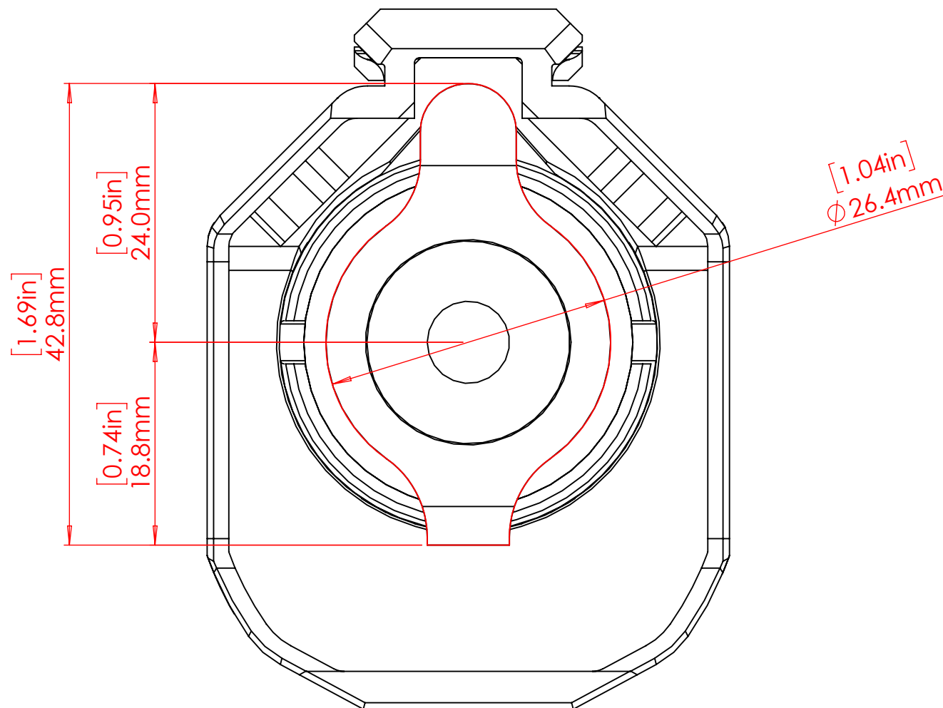
MAXIMUM GAS BLOCK SIZE
