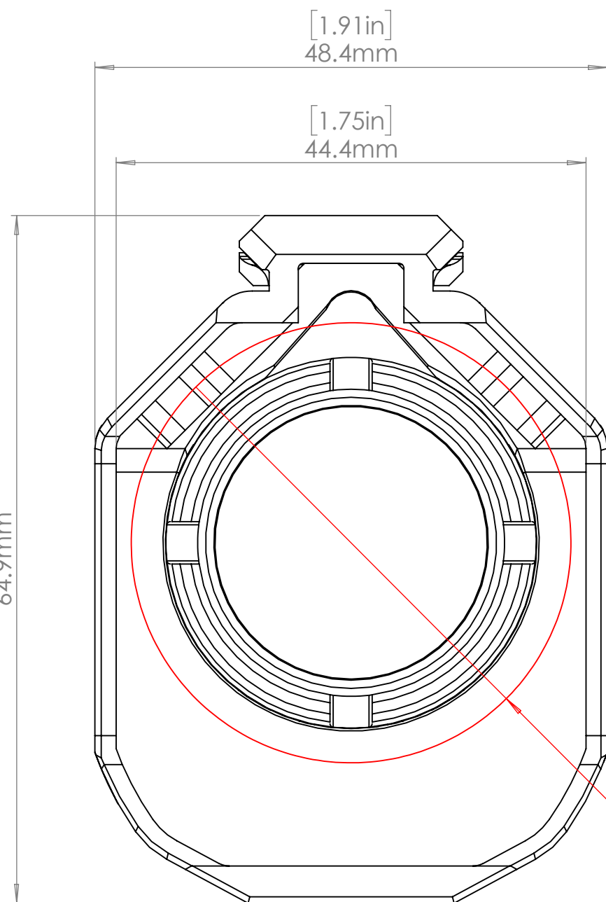
MAXIMUM SUPPRESSOR DIAMETER
